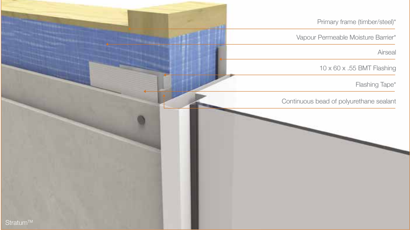
Figure 16 Stratum™ / Stratum™ Duo / Stratum™ Trio Window Jamb
